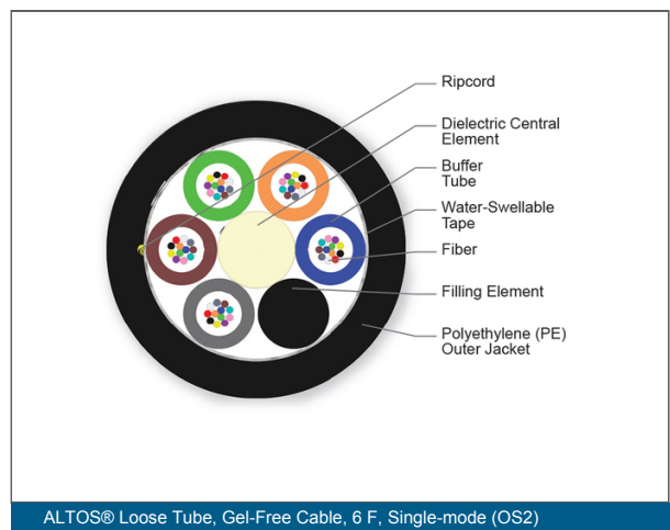
ALTOS® Loose Tube, Gel-Free Cable, 6 F, Single-mode (OS2)
