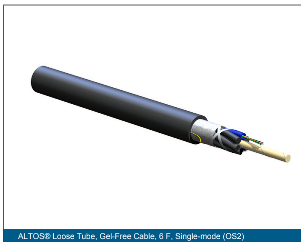
ALTOS® Loose Tube, Gel-Free Cable, 6 F, Single-mode (OS2)
